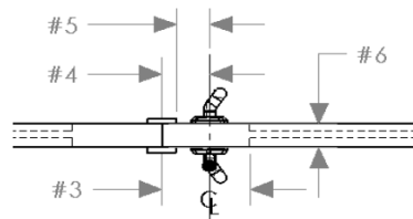
SLIDING DOOR PLAN VIEW
